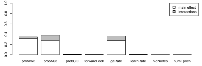
(b) Sensitivity analysis of the selected metamodel
