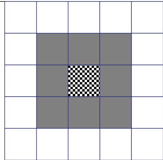
Moore Neighborhood
