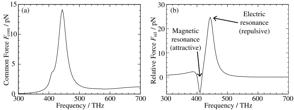
Fig. 2. (a) The common and (b) the relative optical force exerted on a pair of nanowires by an incident field of 50 mW/ \mu\text{m}^2 . The length of the nanowires is L = 100 nm, their diameter is D = 25 nm, and the distance between the nanowires is d = 25 nm. The relative force exhibits two resonances: the magnetic dipole resonance with an attractive force and the electric dipole resonance with a repulsive force.
