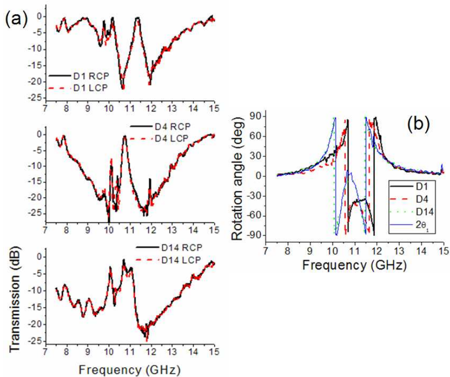
Fig. 4. Experimental results: (a) The transmission spectra of RCP and LCP waves through two chiral layers for three different configurations; (b) The polarization rotation angle of two chiral layers and the doubled polarization rotation angle of a single chiral layer.
