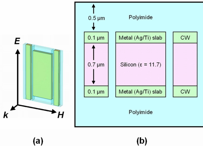
Fig. 1. (a). A single unit cell of the slab-pair metamaterial under study, (b) k-H cross section of the slab-pair metamaterial, passing through the middle of the u.c. along \mathbf{E} direction (metal thickness 0.1\mu\text{m} , polyimide 0.5\mu\text{m} , Silicon 0.7\mu\text{m} ). The figure scaling in the two different dimensions is dissimilar. CW denotes the continuous wires.
