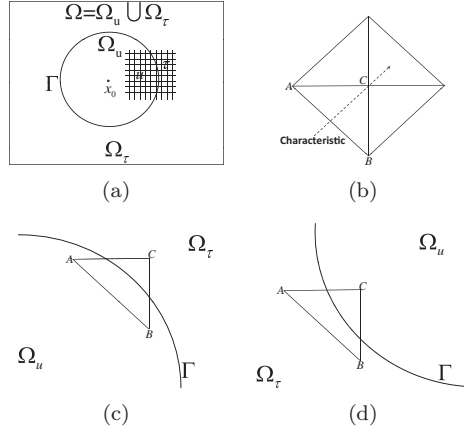
FIG. 3.1. Domain and mesh (2-D). (a) Domain \Omega and different regions \Omega_u and \Omega_\tau . (b) Local mesh of point C . (c) and (d) A triangle/simplex across two regions, \Omega_u and \Omega_\tau .
