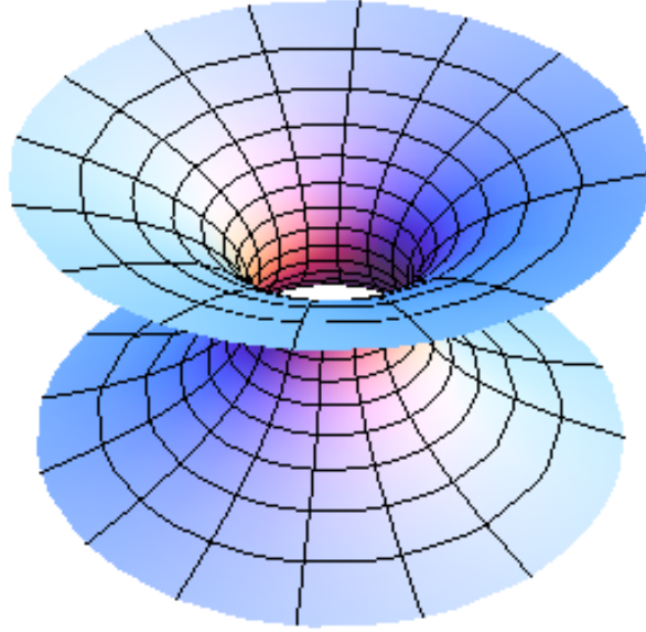
Figure 2: Catenoid (2 \cos u \cosh(v/2), 2 \sin u \cosh(v/2), v) over [0, 2\pi] \times [-4, 4] .
