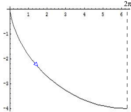
Figure 1: The cycloid 2(\theta - \sin \theta, \cos \theta - 1) with 0 \leq \theta \leq \pi is the minimum time trajectory along which a particle starting at the origin slides pass the vertical line x = 2\pi under gravity.
