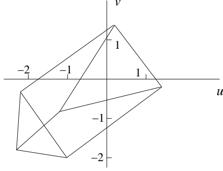
Figure 8: Projected prism in Figure 5 in viewplane coordinates.
