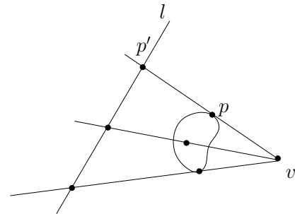
Figure 1: Perspective Projection
