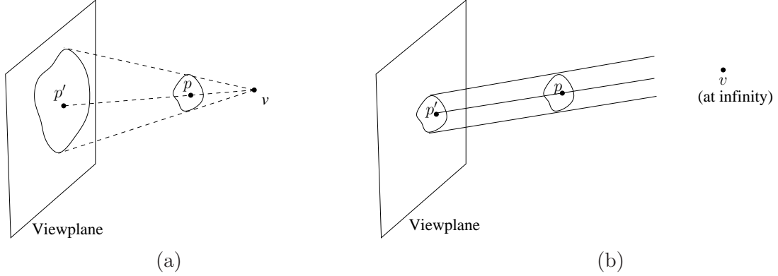
Figure 4: (a) Perspective projection and (b) parallel projection.
