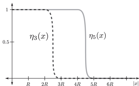
FIG. 2. The cutoff functions \eta_3(x) and \eta_5(x) .
