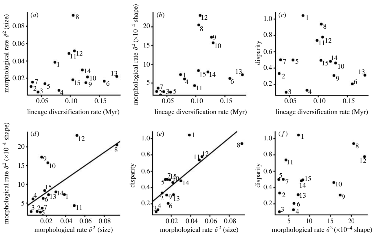
Figure 2. Relationships between rates of morphological size evolution, morphological shape evolution and species diversification among 15 clades of plethodontid salamanders (clade numbers follow table 1). (a) Diversification rate versus rate of size evolution; (b) diversification rate versus rate of shape evolution; (c) diversification rate versus morphological disparity; (d) rate of size versus shape evolution; (e) rate of size evolution versus morphological disparity; and (f) rate of shape evolution versus morphological disparity. Only significant regressions are displayed. Full results are provided in table 2.
