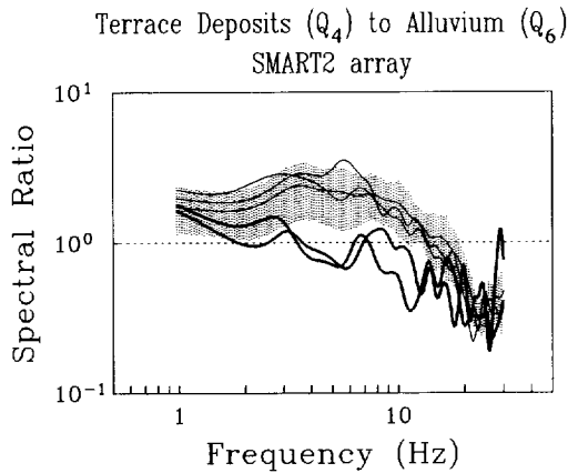
Fig. 7. Spectral ratios between stations 3 and 36 of the SMART2 array. Ratios are shown for weak (thin lines) and strong (thick lines) excitation strengths.
