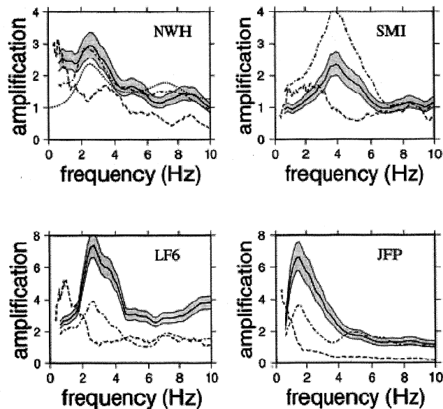
Figure 11. Site response estimates at four sites that reveal a clear fundamental resonance in the weak-motion estimate (solid lines with 95% confidence intervals shaded). The dot-dashed lines represent average horizontal to vertical component spectral ratios, and the dotted line for NWH is the predicted one-dimensional weak-motion shear wave site response based on a borehole study at the site (preliminary data from the "Resolution of Site Response Issues from the Northridge Earthquake" project; C. Roblee, personal communication, 1997). The horizontal to vertical component spectral ratios, and the theoretical prediction, provide independent evidence that the observed peaks represent a fundamental resonance of the sediments. That the peaks are clearly absent, or at least shifted, in the strong motion estimates (dashed lines), suggests a nonlinear response during the main shock.
