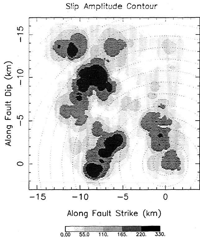
Figure 7. The Northridge earthquake net slip distribution, reproduced from Zeng and Anderson [1996] , used to compute the main shock synthetic seismograms. The dotted lines are contours of rupture time at 0.5-s intervals. © 1996, Seismological Society of America. All rights reserved.
